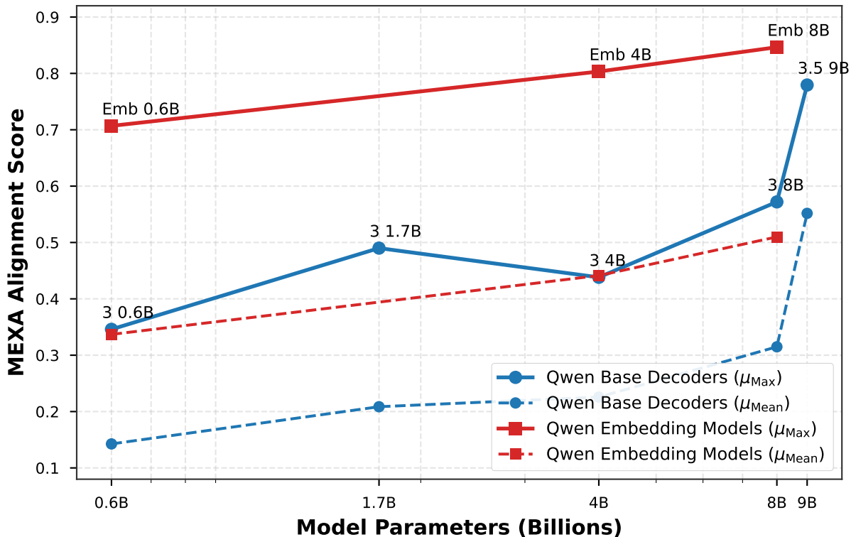
Parameter Scaling of Cross-Lingual Alignment in Qwen Family
